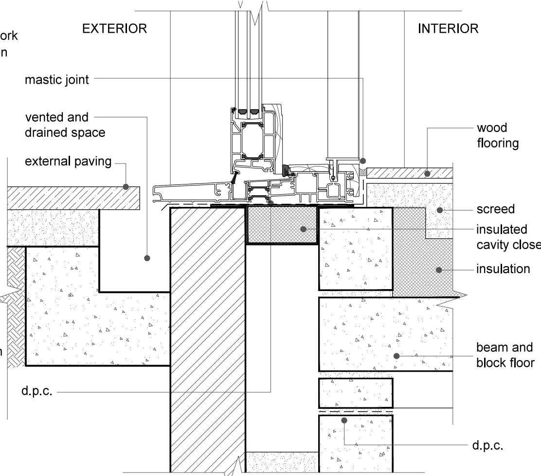
3 sill detail - level paving
